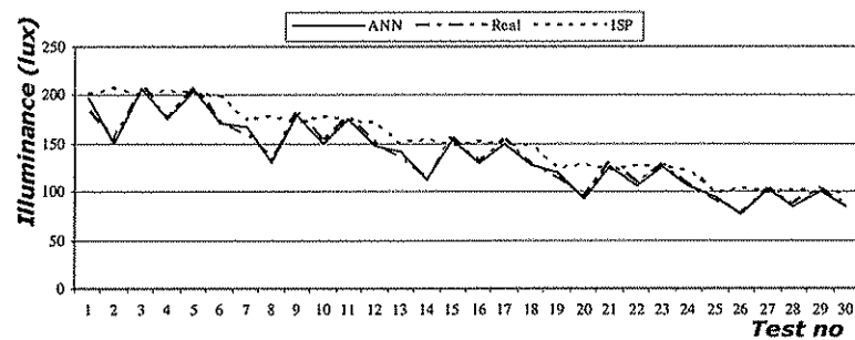
Fig. 9. Results of the testing step; ANN, real and ISP output values of minimum illuminance
