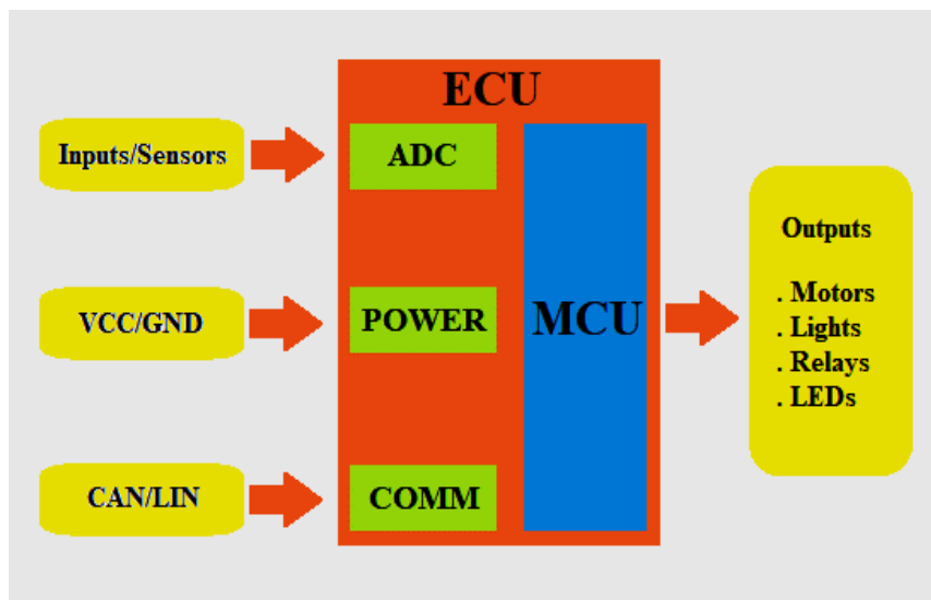
Figure 2. Structure of ECUs.
