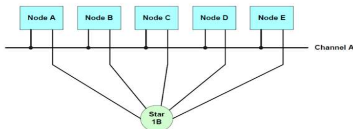
Figure 20. Hybrid topologies of FlexRay (FlexRay Protocol Specification, 2005).
