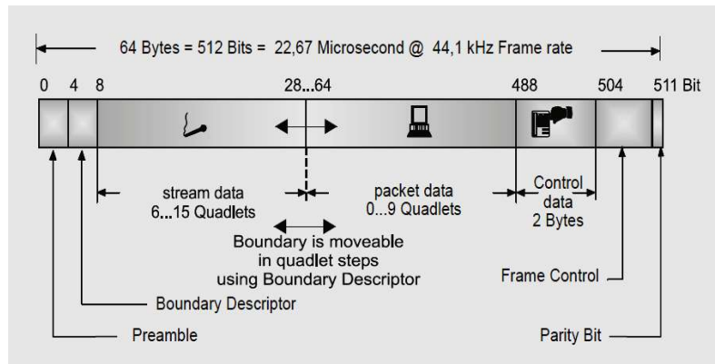
Figure 25. Frame of MOST25 (MOST Specification, 2005).
