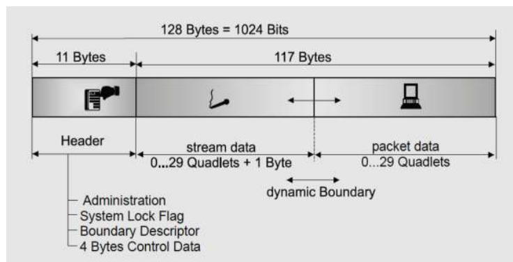
Figure 26. Frame of MOST50 (MOST Specification, 2005).
