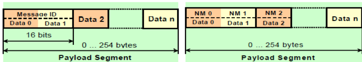
Figure 22. Static and Dynamic segment (FlexRay Protocol Specification, 2005).
