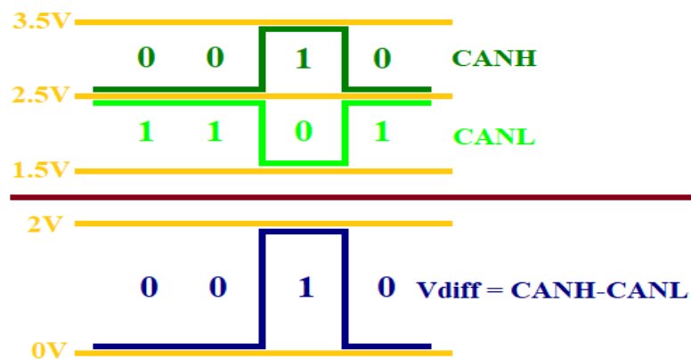
Figure 14. CAN signal voltage level.
