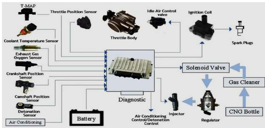
Figure 4. Engine Control Unit (ECU) Structure (ECU Engine Control Unit, 2020).
