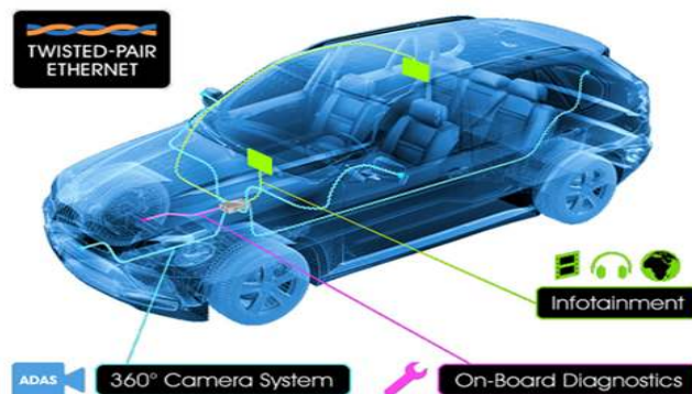
Figure 28. Ethernet network in vehicle (Automotive Ethernet Technology, 2017).
