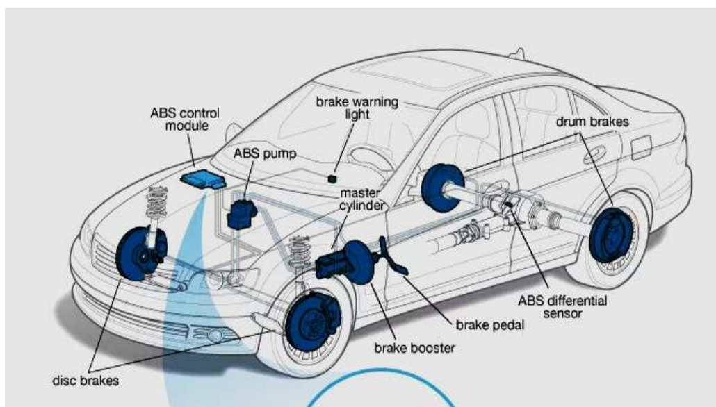
Figure 7. Anti-Lock Braking System (ABS Control Module, 2020).
