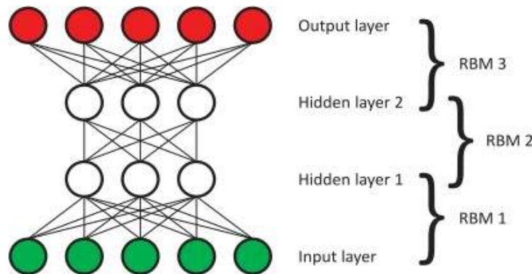
Figure 3. DBN Architecture.
