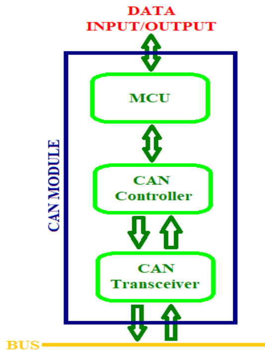
Figure 13. CAN module.
