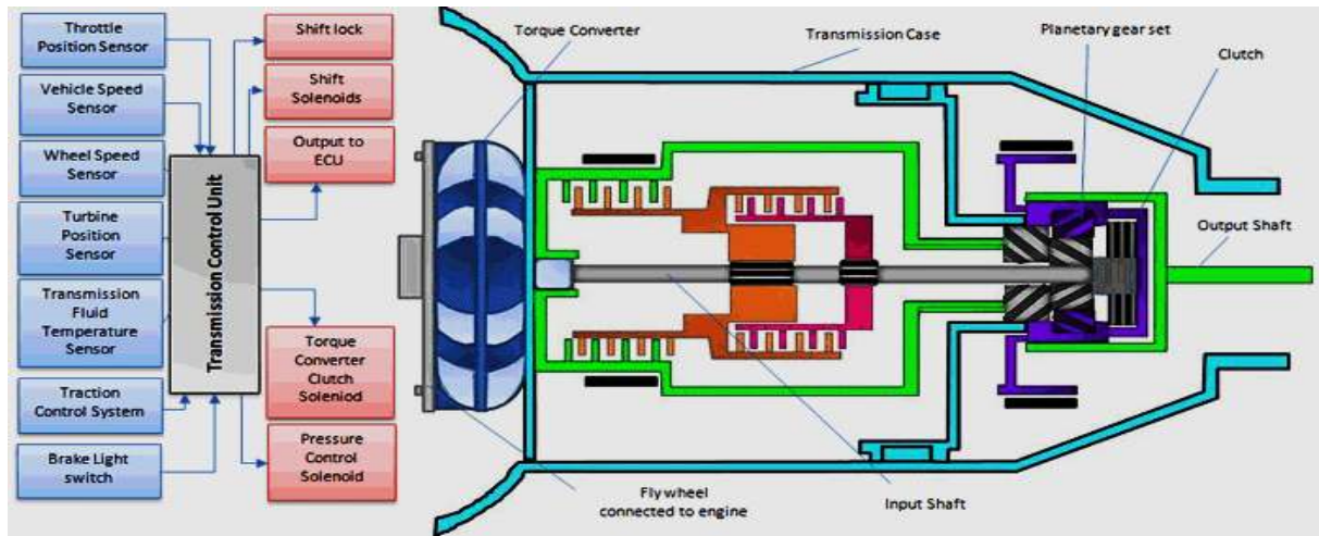
Figure 5. Component of Transmission Control Unit (Transmission Control, 2020).
