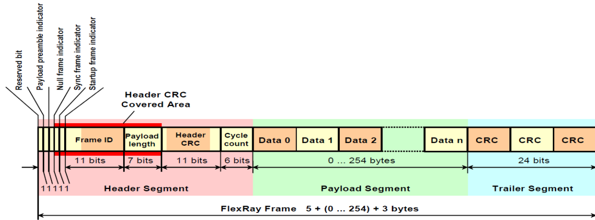
Figure 21. Structure of frame in FlexRay (FlexRay Protocol Specification, 2005).
