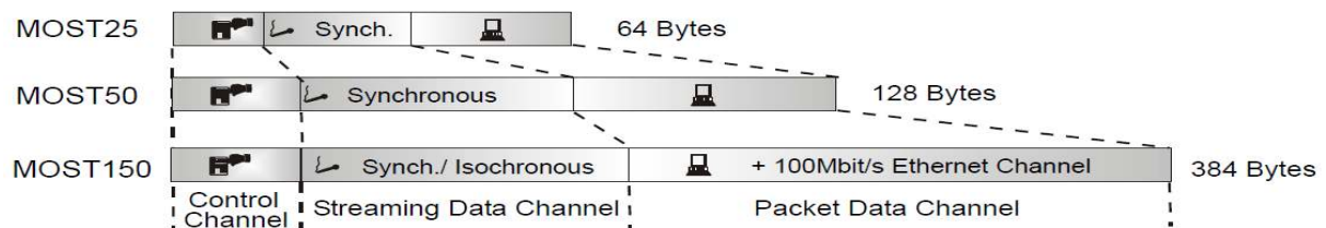
Figure 24. Comparing MOST versions (MOST Specification, 2005).
