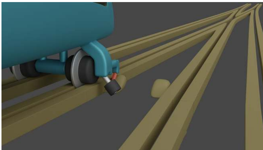
Figure 4. Interception. Example of a mechanical safety measure to ensure the right position of the channelling wheels
