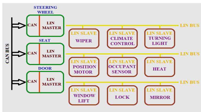
Figure 10. Example of CAN and LIN bus system.
