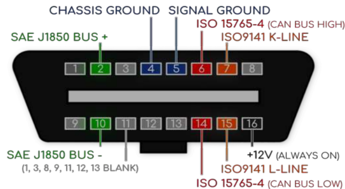
Figure 30. OBD2 Socket pinout (OBD2 Explained-A simple intro, 2020).
