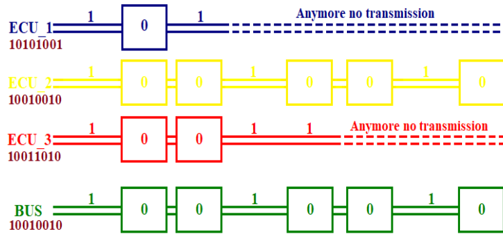
Figure 15. CAN bus arbitration.
