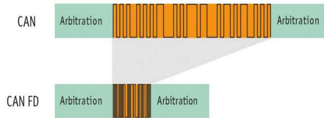
Figure 19. Comparing CAN and CAN FD (CAN FD, 2018).
