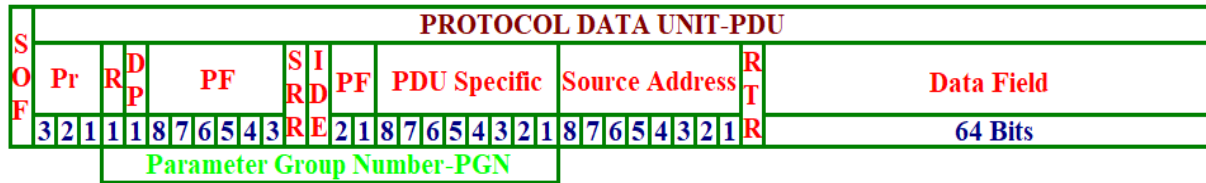
Figure 32. Frame of SAE J1939.
