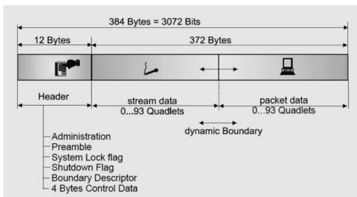
Figure 27. Frame of MOST150 (MOST Specification, 2005).
