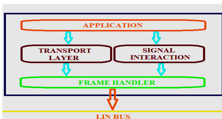
Figure 9. LIN module.
