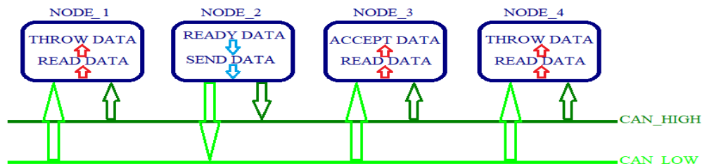
Figure 12. Data broadcasting of CAN.
