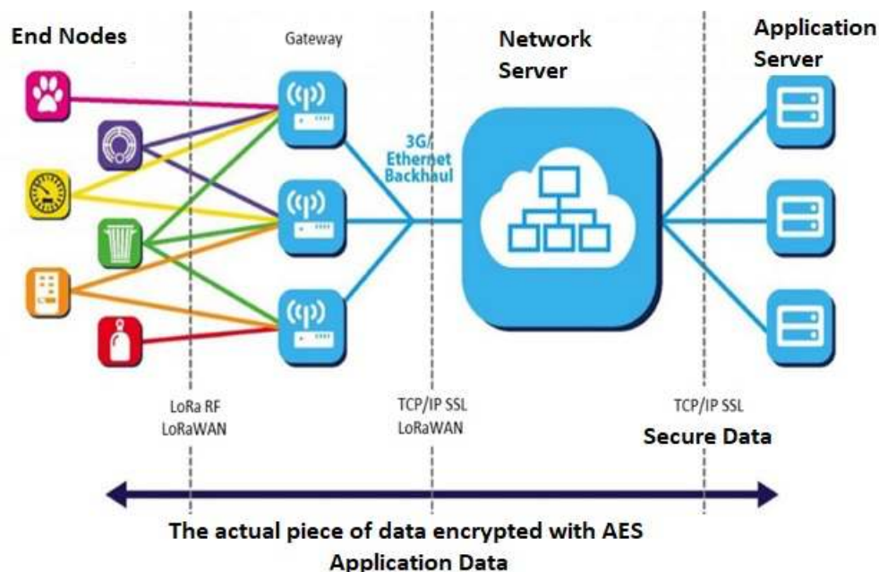
Figure 2. LoRa Communication Technology Structure [25]
