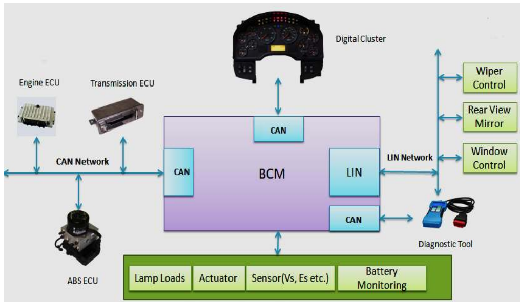
Figure 3. Link of Body Control Unit with other (Body Control Module, 2020).
